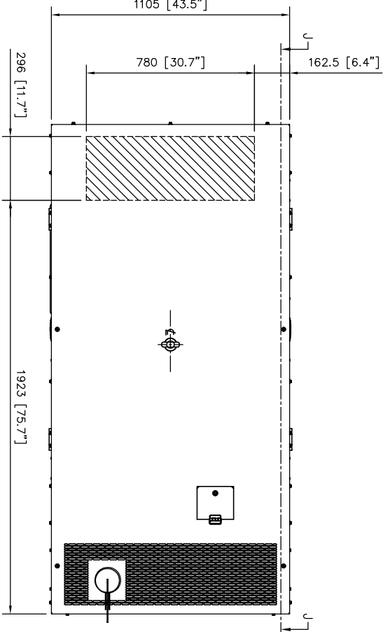
TANKBASE PLAN SHOWING SOCKET LAYOUT
